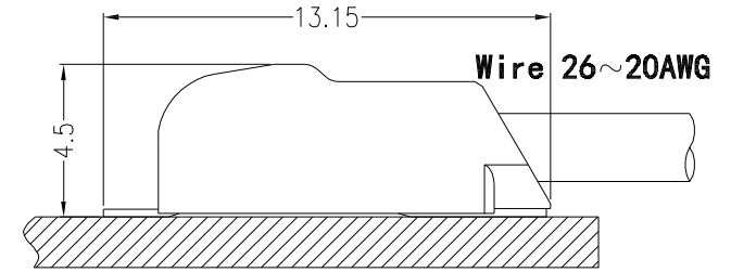
Installation drawing
