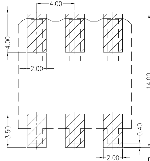
Board Layout
