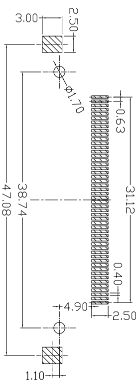
Recommended P.C.B Layout(Top Side)
