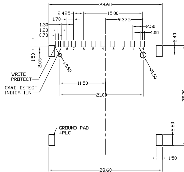
RECOMMEND P.C.B LAYOUT (TOLERANCES ±0.10mm)
