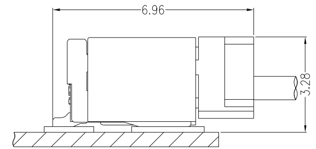
Assembly Layout
